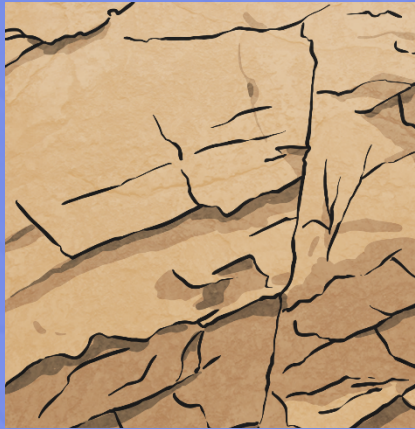
Igneous
